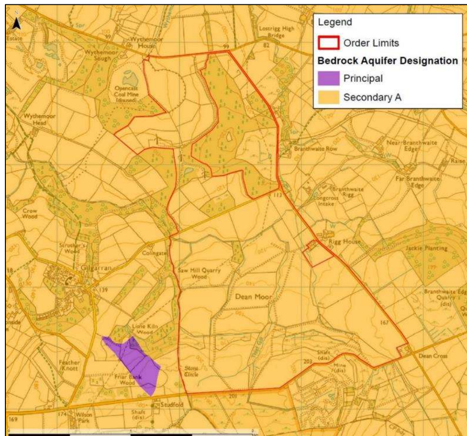
Figure 3.3: Bedrock Aquifer Designation
