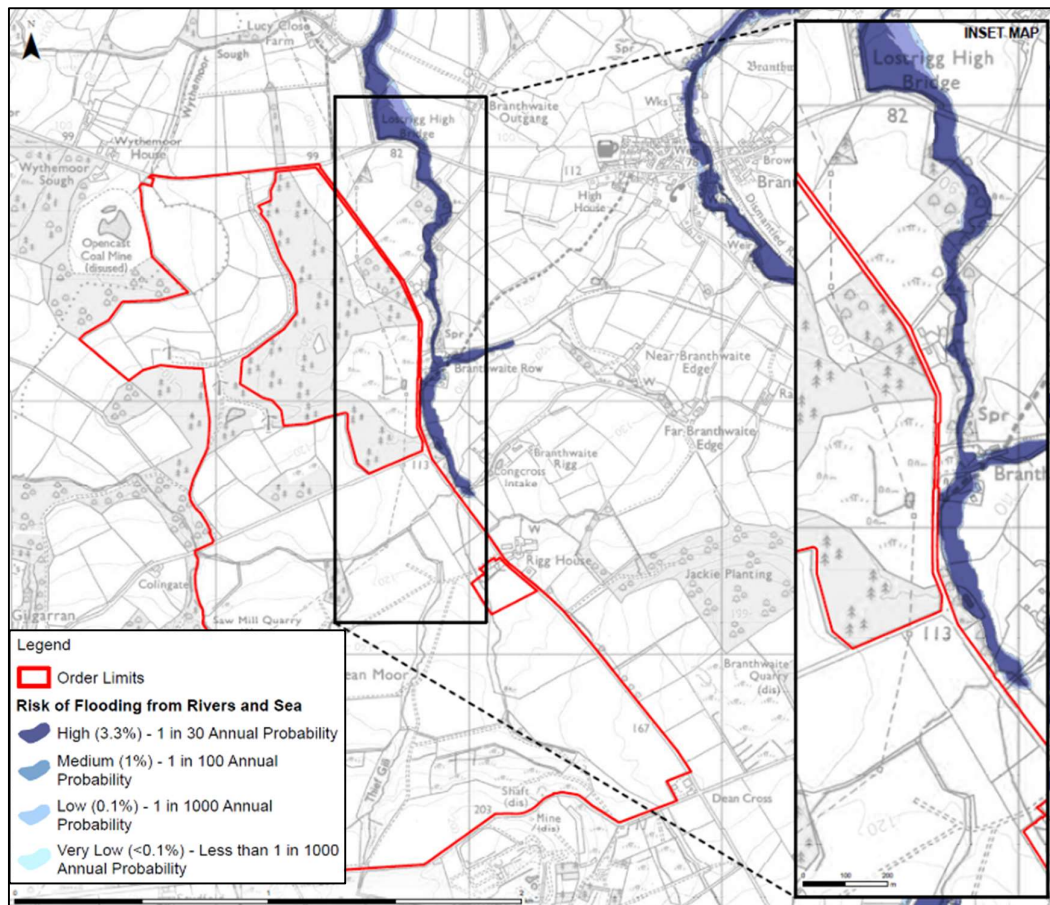
Figure 5.2: Fluvial Flood Risk Map (incl. climate change)
