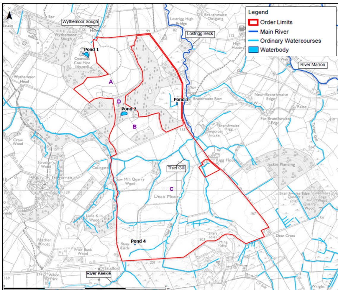
Figure 3.1: Hydrological Context of Site
