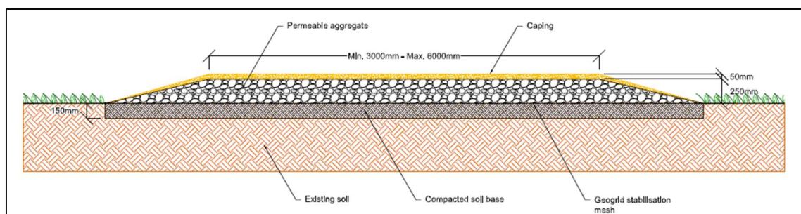
Figure 8.8: Typical No Dig Internal Access Track
