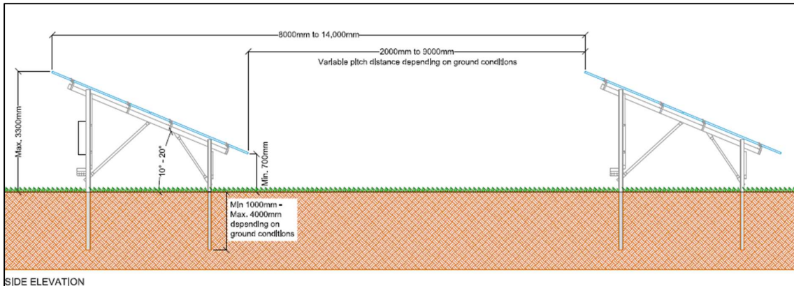
Figure 8.1: Array Framework Structure Cross Section (Standard)
