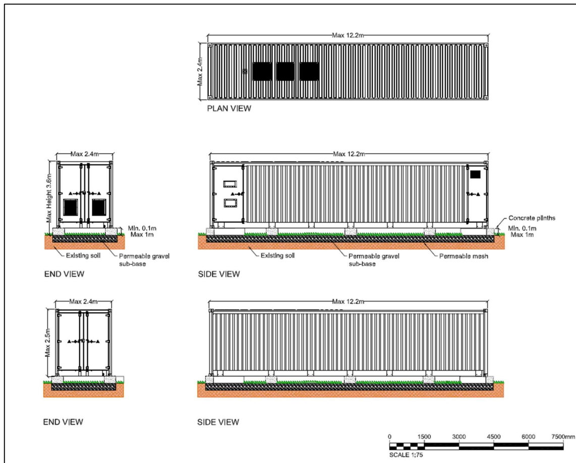
Figure 8.6: Indicative PCS Unit
